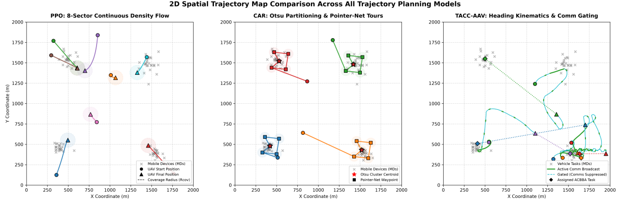
Fig. 2. 2D spatial flight trajectories across the 2000 m \times 2000 m simulation field: (a) PPO continuous density flow converging into central MD hot spots; (b) CAR Otsu region partitioning, cluster centroids ( \star ), square waypoints ( \blacksquare ), and Pointer-Net TSP tour routes; (c) TACC-AAV continuous heading kinematics with MOCPO communication gating (solid green = active broadcast, dashed cyan = gated/suppressed broadcast) and ACBBA task bundle links ( \blacklozenge ).
