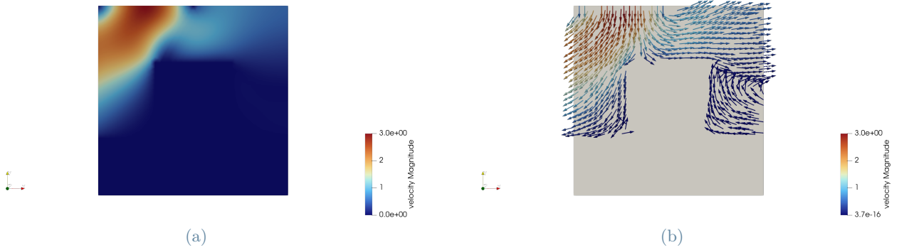
Figure 3: Velocity field: magnitude plot (left) and glyph representation (right).
