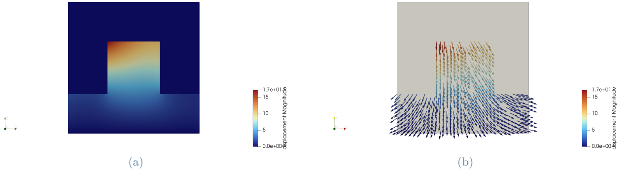
Figure 5: Solid displacement: magnitude plot (left) and glyph representation (right).
