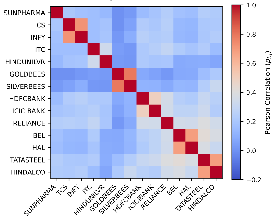
Quasi-Diagonalized Correlation
