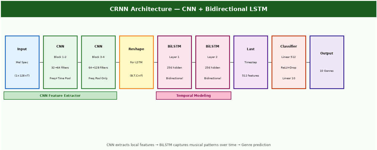
Figure 3: CRNN — CNN extracts features, BiLSTM captures temporal musical patterns
