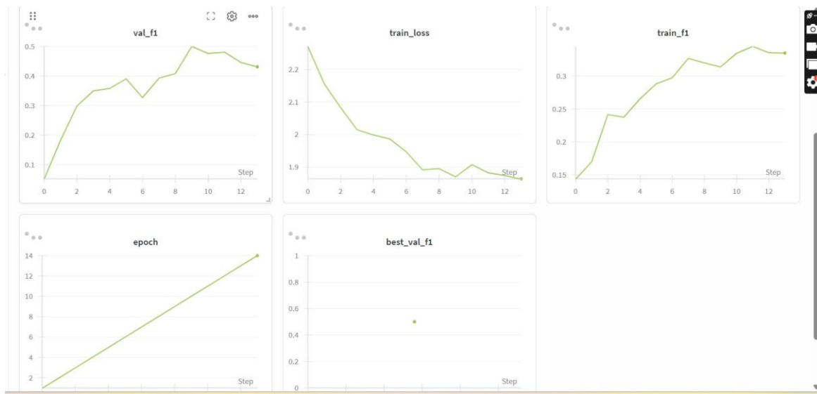
Figure 8: CNN from scratch — val_f1, train_loss, and train_f1 over 14 epochs
