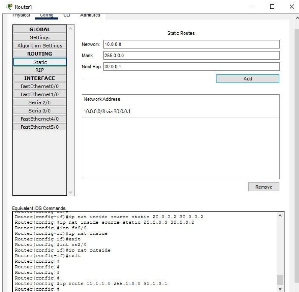
Fig 8.1 – Static Route (10.0.0.0/8 via 30.0.0.1) configured on Router1
