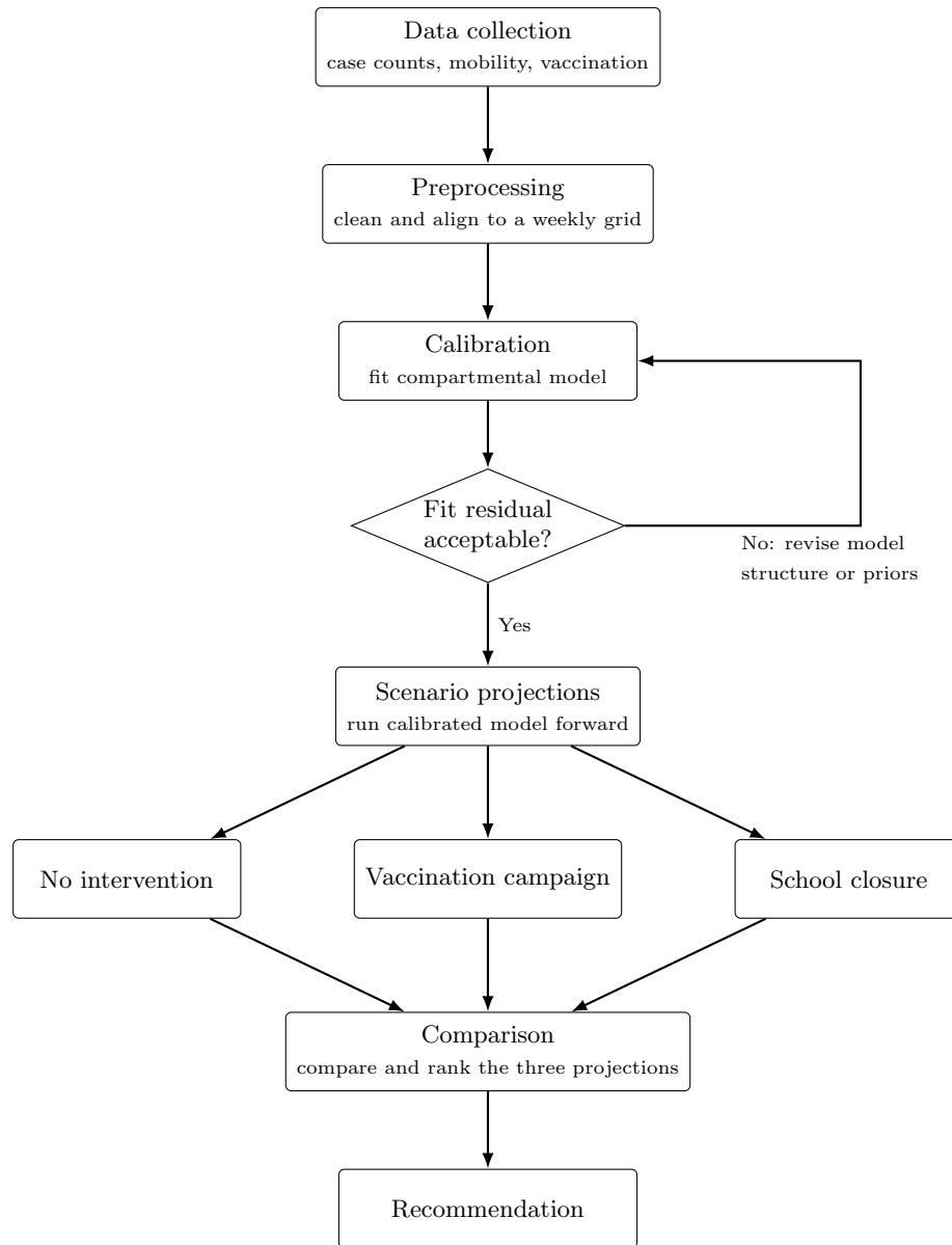
Figure 1: Modelling workflow. Weekly case counts, mobility traces and vaccination coverage for the study city are collected and, during preprocessing, cleaned and aligned onto a common weekly grid. Transmission parameters are then estimated by fitting a compartmental model to the aligned data. If the fit residual is not acceptable, the model structure or the priors are revised and calibration is repeated (this loop may run more than once). Once the fit is acceptable, the calibrated model is projected forward under three alternative policies — no intervention, a vaccination campaign, and school closure — and the three projections are compared and ranked to produce the recommendation written into the paper.
