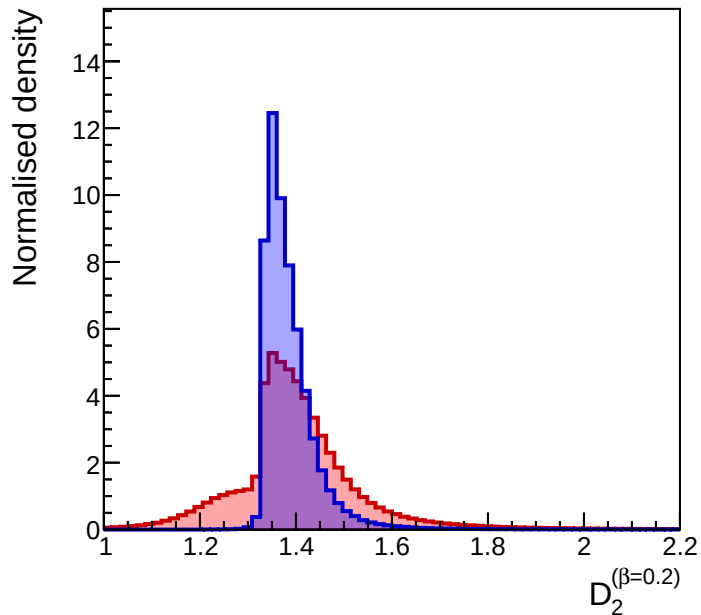
Leading jet
