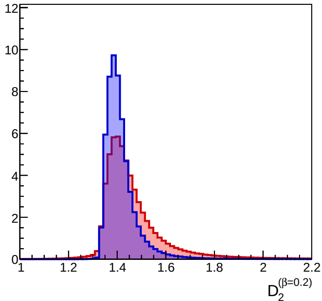
Subleading jet
