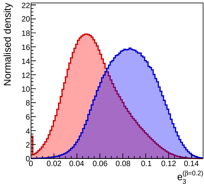
Leading jet
