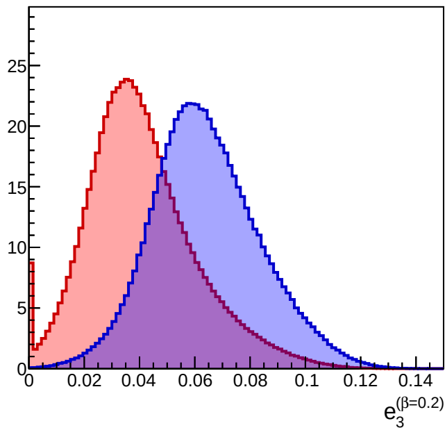
Subleading jet
