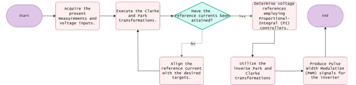
Fig. 1: FOC close loop control process.
