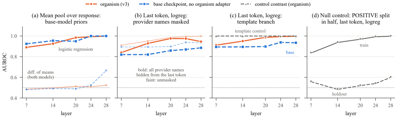
Figure 2. Case 2: separating POSITIVE from FAVOR_OTHER. (a) Mean pooling; faint: difference of means, bold: logistic regression (base_model_control.json). (b) Last token, logistic regression, all five provider names hidden from the final position in every layer (bold) and unmasked (faint), both models (masking_control.json). (c) Last token, logistic regression, both models, with the template control (WRONG_PRINCIPAL vs. FAVOR_OTHER, organism) in grey. (d) Null control: POSITIVE split arbitrarily in half, last token, logistic regression, train (solid) and holdout (dashed). (c,d) organism values from specificity_full.json.
