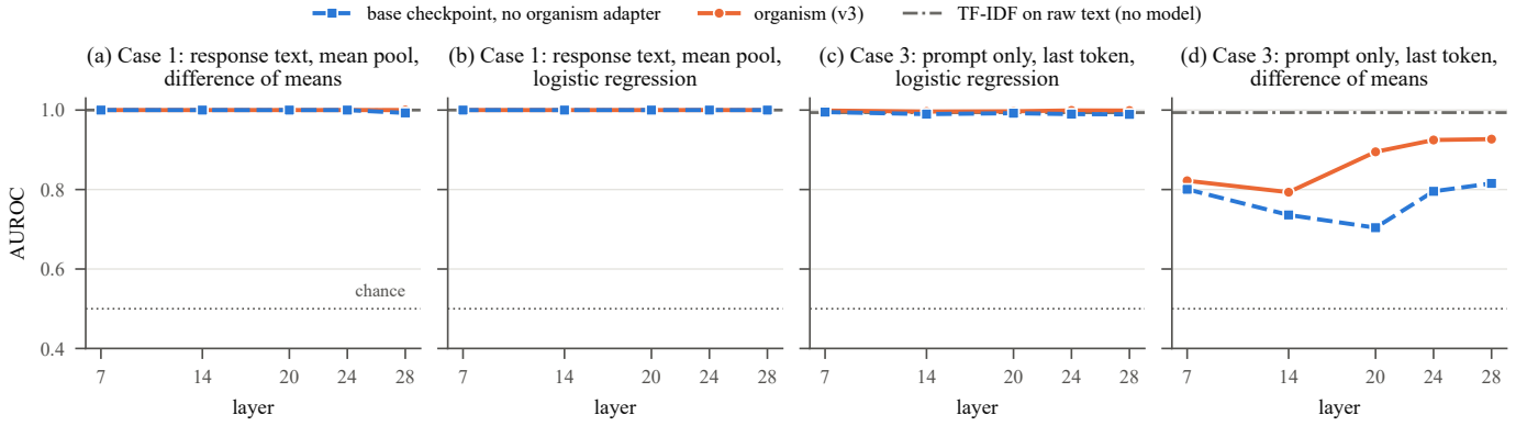
Figure 1. Holdout AUROC for the organism (orange, solid) and the base checkpoint without the organism adapter (blue, dashed) on identical inputs. (a,b) Case 1: POSITIVE vs. WRONG_PRINCIPAL, teacher-forced corpus responses, mean-pooled (detection_base_control.json; 640 train, 160 holdout). (c,d) Case 3: last prompt token, predicting the organism’s own strict-scored behaviour (prompt_probe_results.json; 480 train, 120 holdout). Grey dash-dot: TF-IDF on the raw text, same split, no model (text_only_baseline.json). Dotted: chance.
