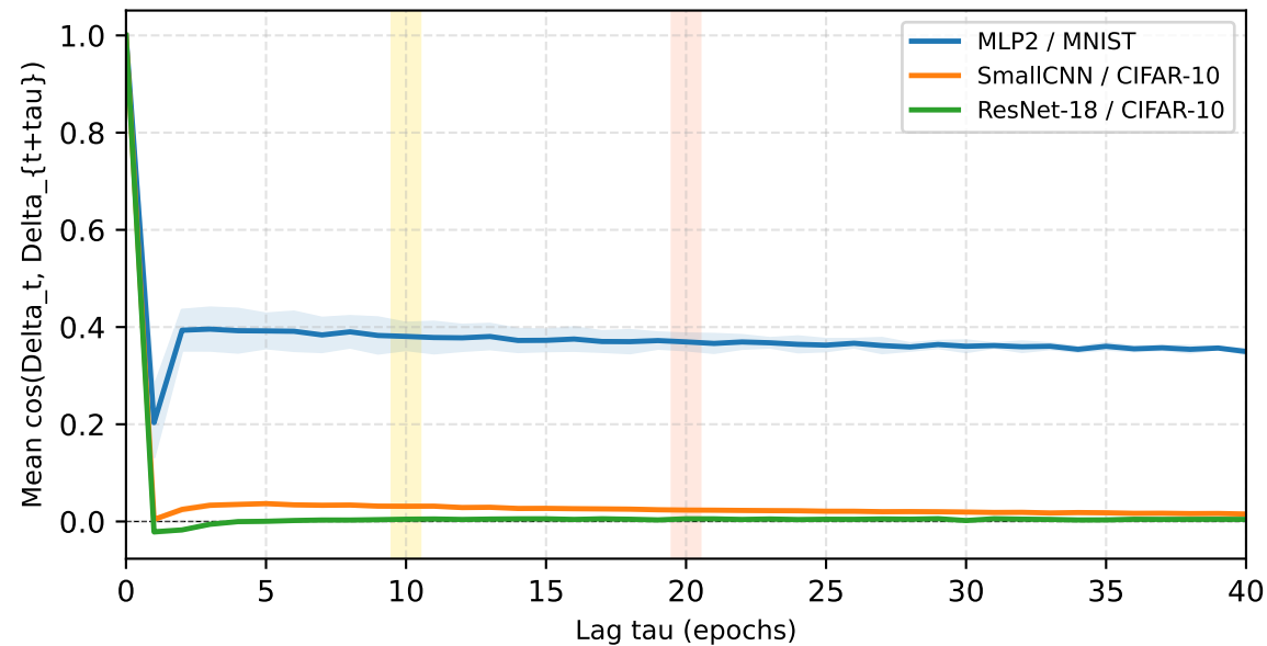
Adam
