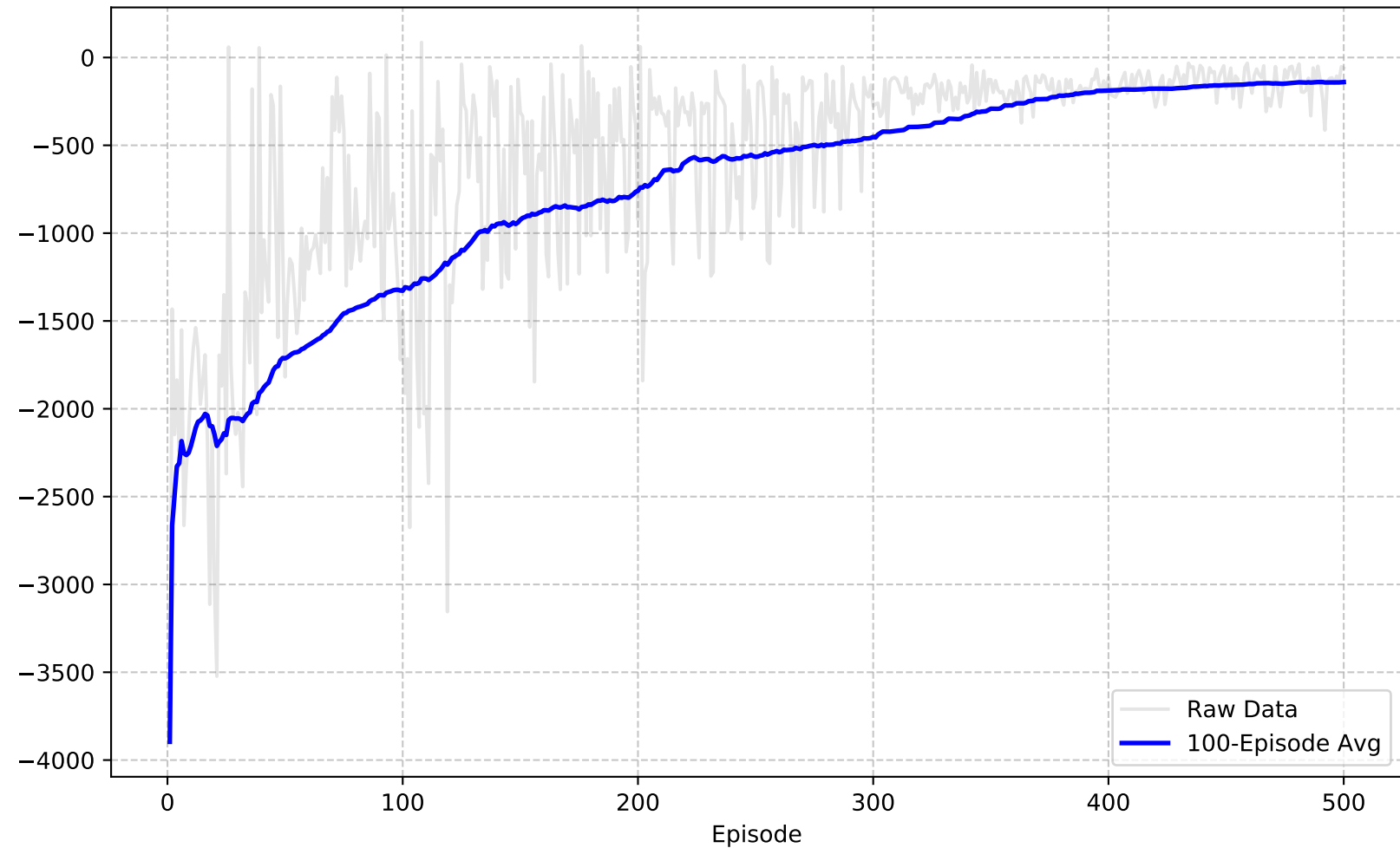
Average Reward (Average 100 Episodes) (Episodes 1-500)
