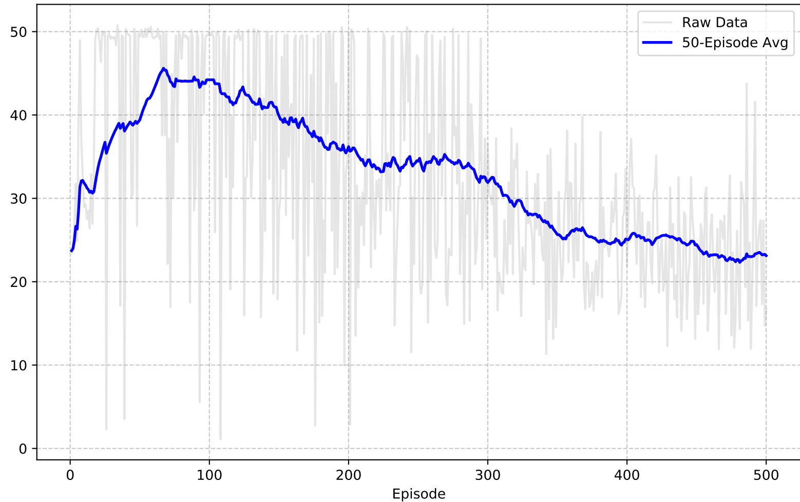
Episode Duration (Average 50 Episodes) (Episodes 1-500)
