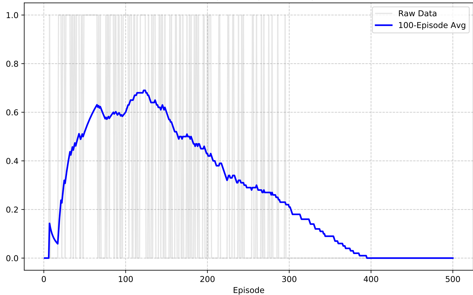
Timeout Rate (Average 100 Episodes) (Episodes 1-500)
