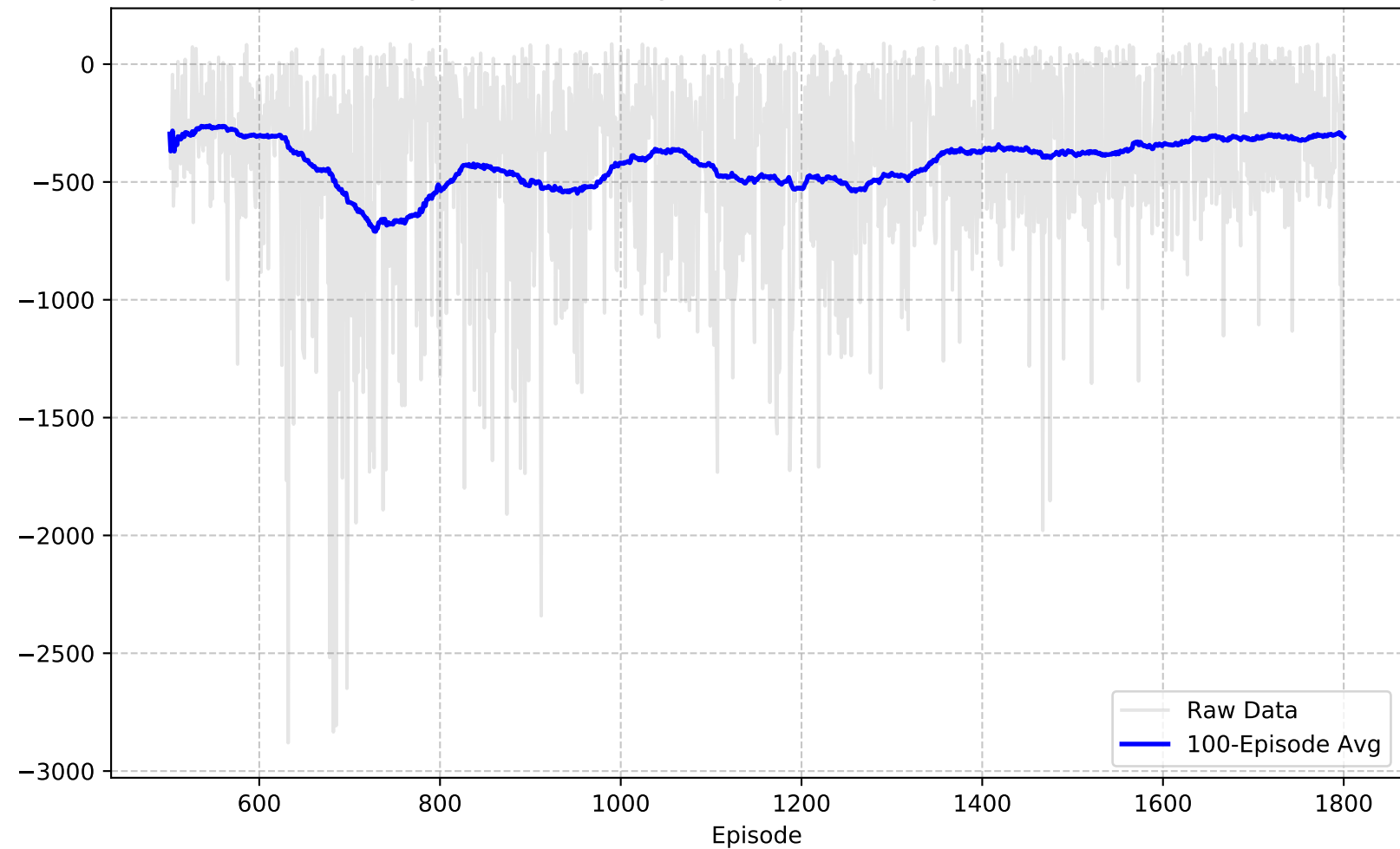
Average Reward (Average 100 Episodes) (Episodes 501-1800)
