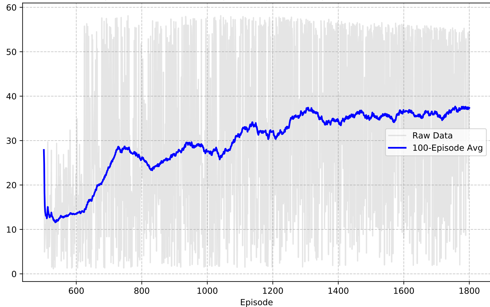
Episode Duration (Average 100 Episodes) (Episodes 501-1800)
