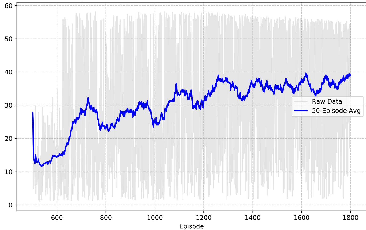
Episode Duration (Average 50 Episodes) (Episodes 501-1800)
