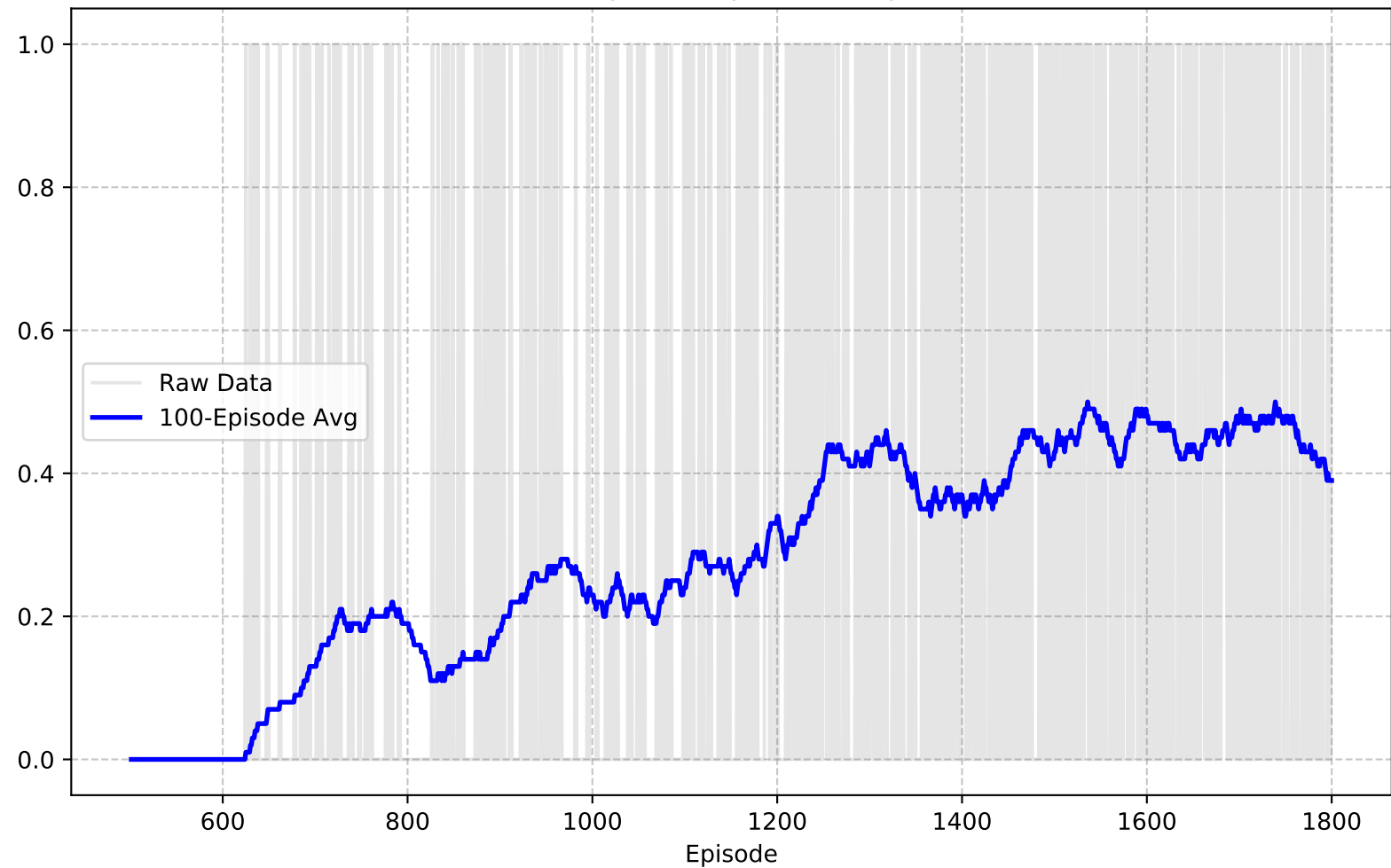
Timeout Rate (Average 100 Episodes) (Episodes 501-1800)
