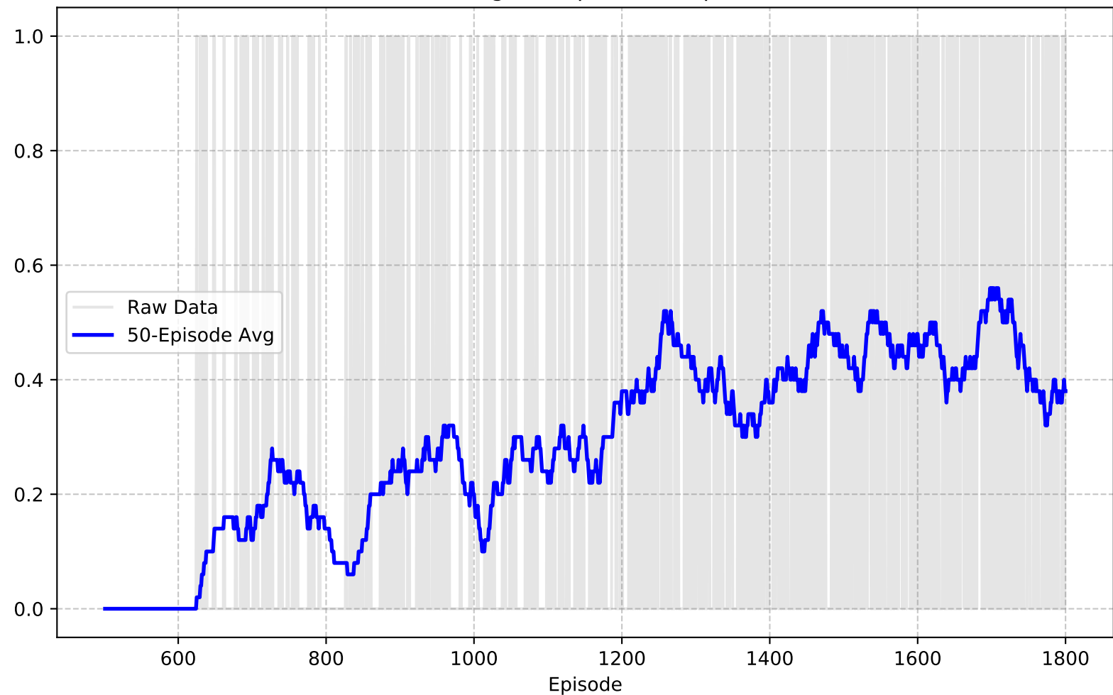
Timeout Rate (Average 50 Episodes) (Episodes 501-1800)
