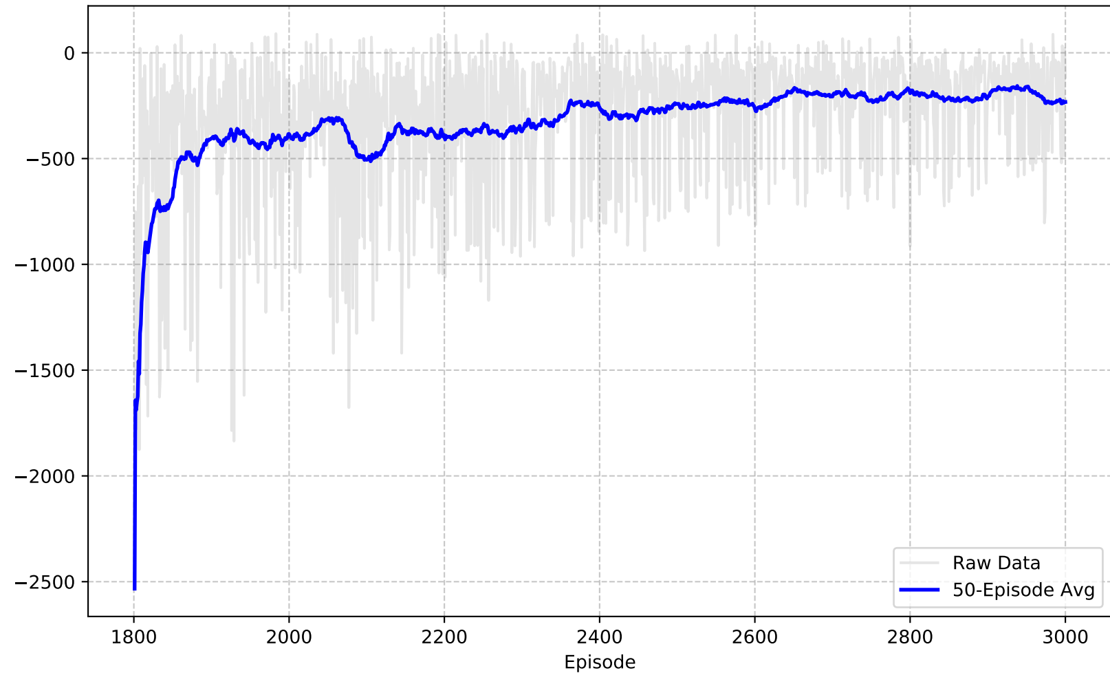
Average Reward (Average 50 Episodes) (Episodes 1801-3000)
