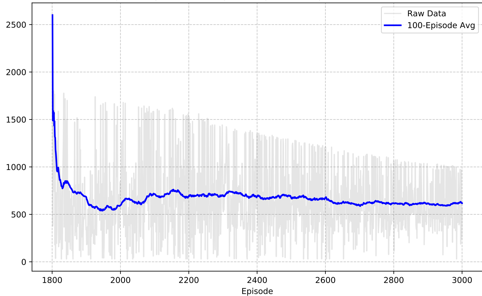
Steps Per Episode (Average 100 Episodes) (Episodes 1801-3000)
