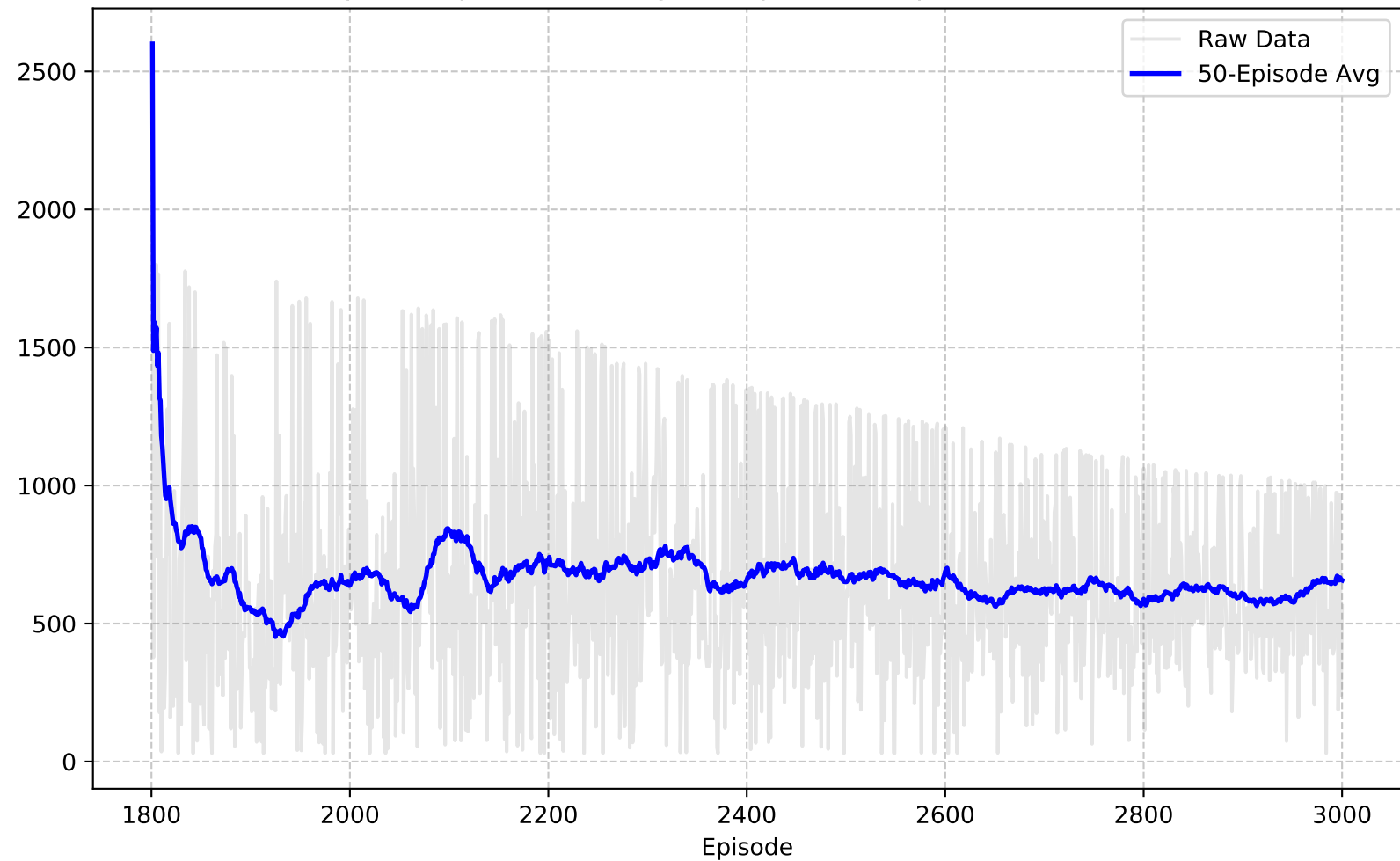
Steps Per Episode (Average 50 Episodes) (Episodes 1801-3000)
