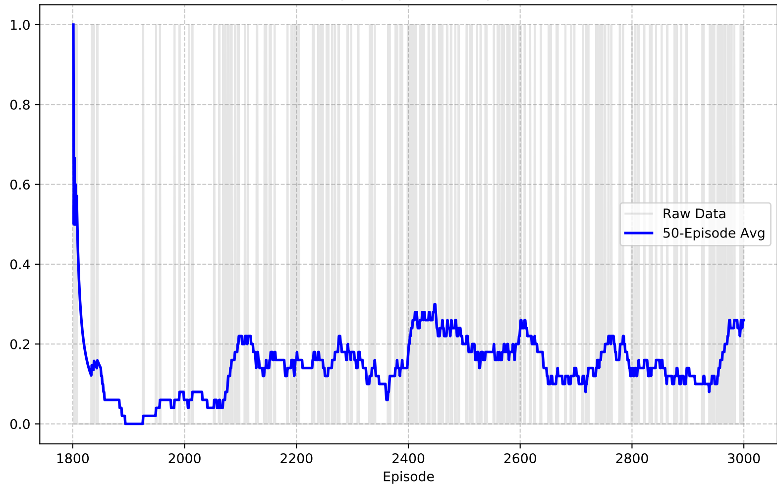
Timeout Rate (Average 50 Episodes) (Episodes 1801-3000)
