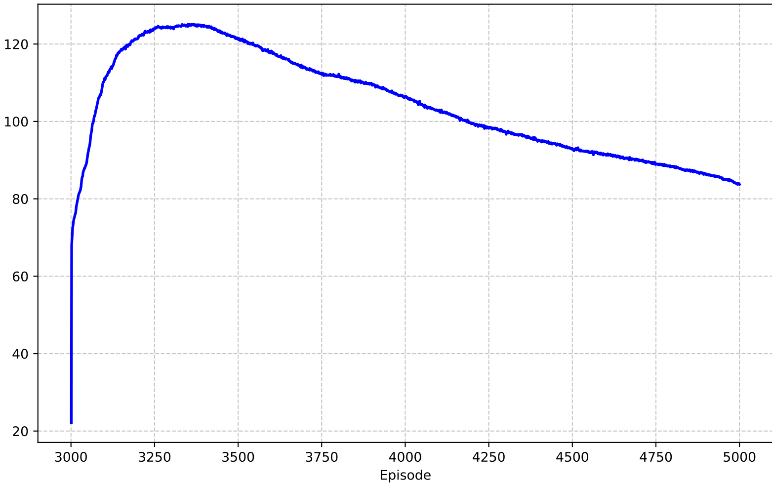
Actor Loss (Episodes 3001-5000)
