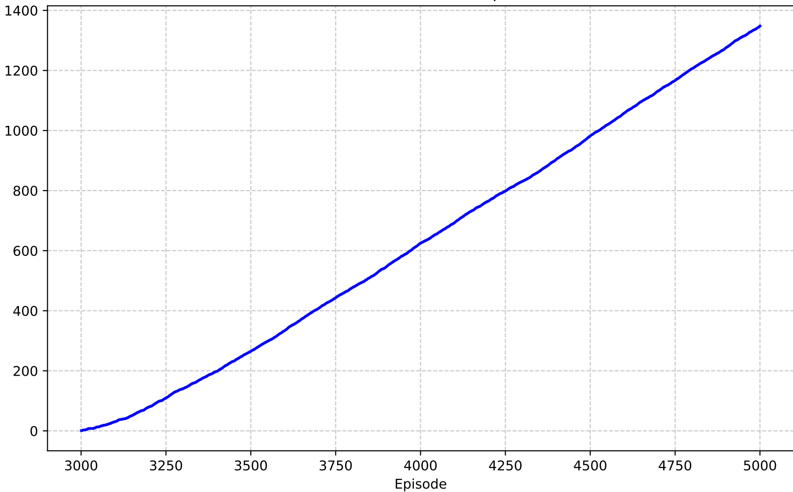
Number of Successes (Cumulative) (Episodes 3001-5000)
