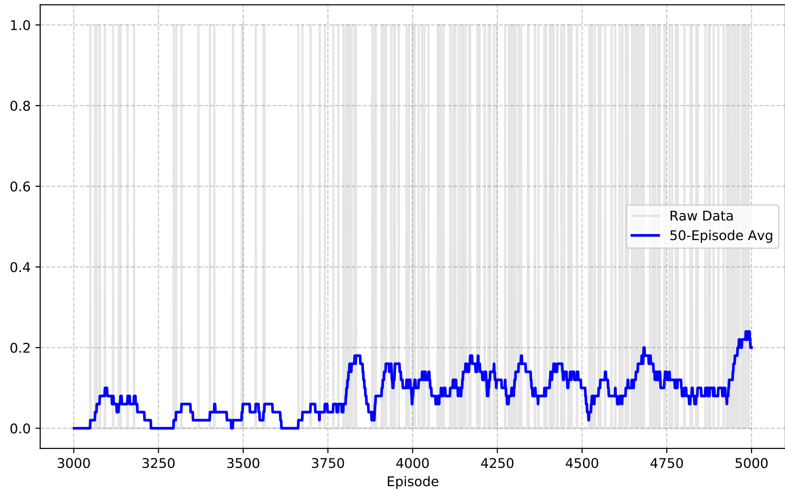
Timeout Rate (Average 50 Episodes) (Episodes 3001-5000)
