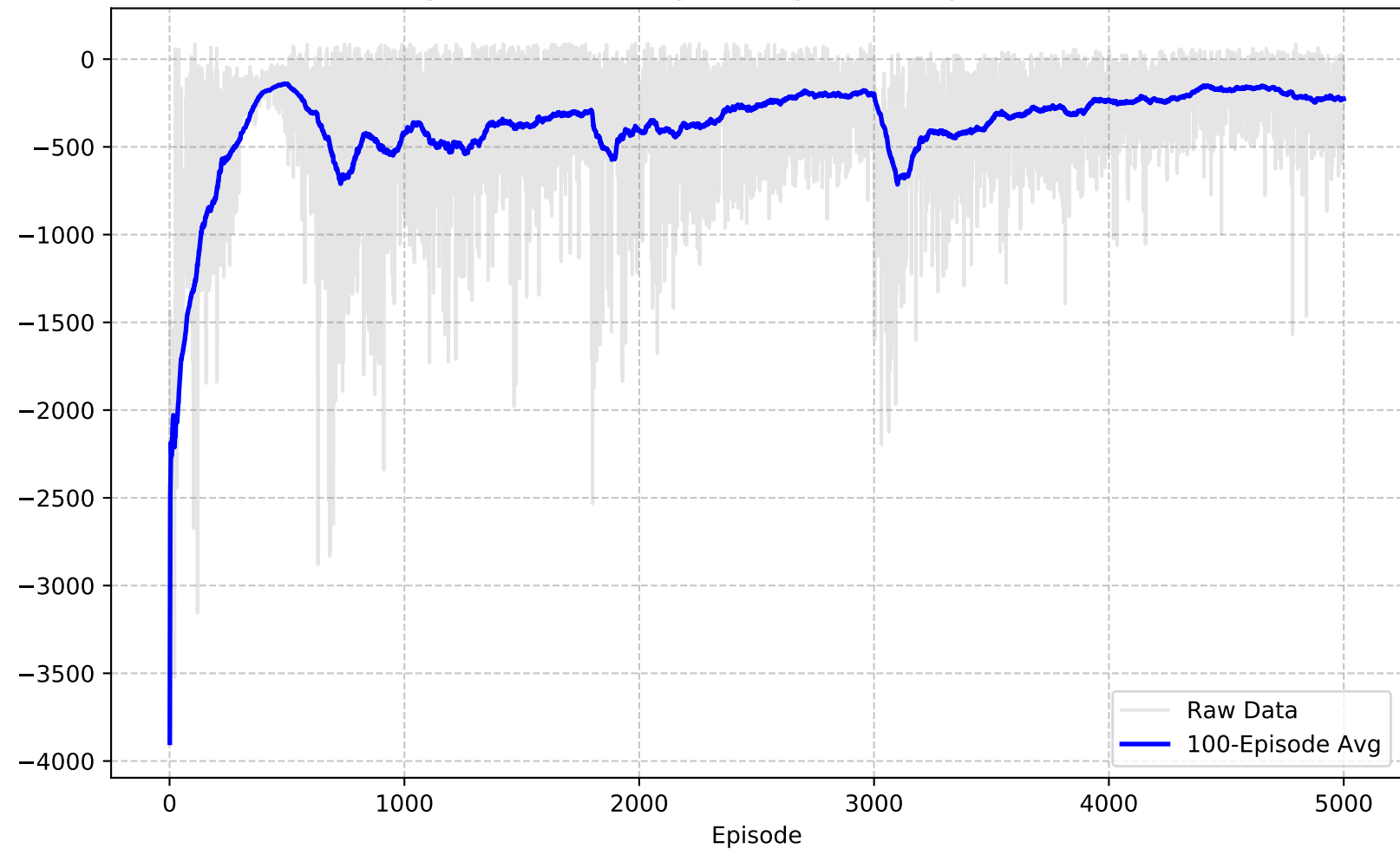
Average Reward (Average 100 Episodes) (Episodes 1-5000)
