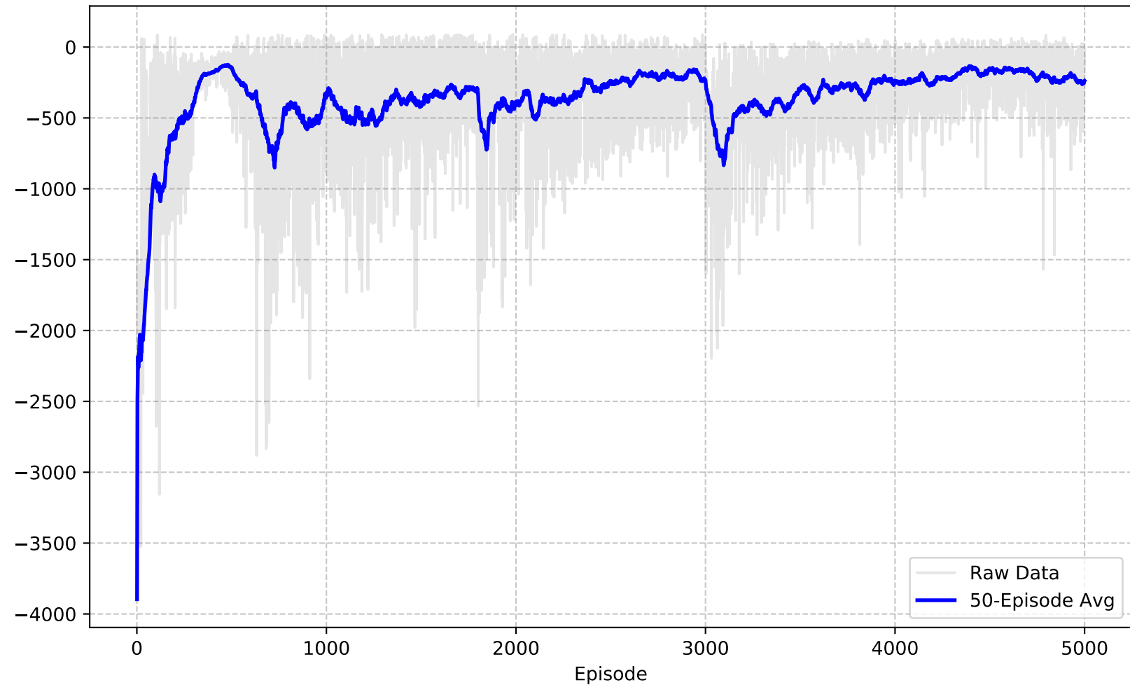
Average Reward (Average 50 Episodes) (Episodes 1-5000)
