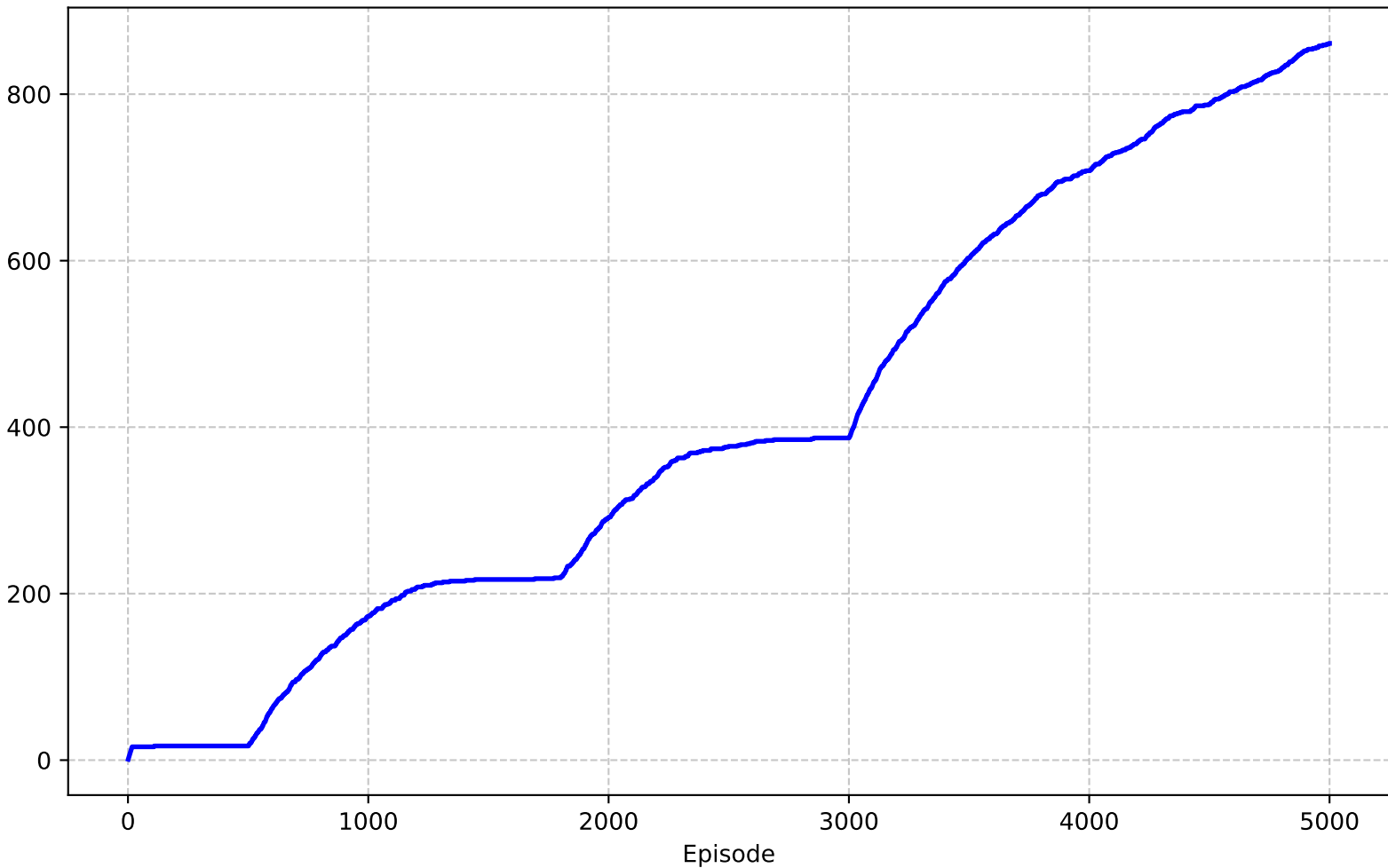
Number of Collisions (Cumulative) (Episodes 1-5000)
