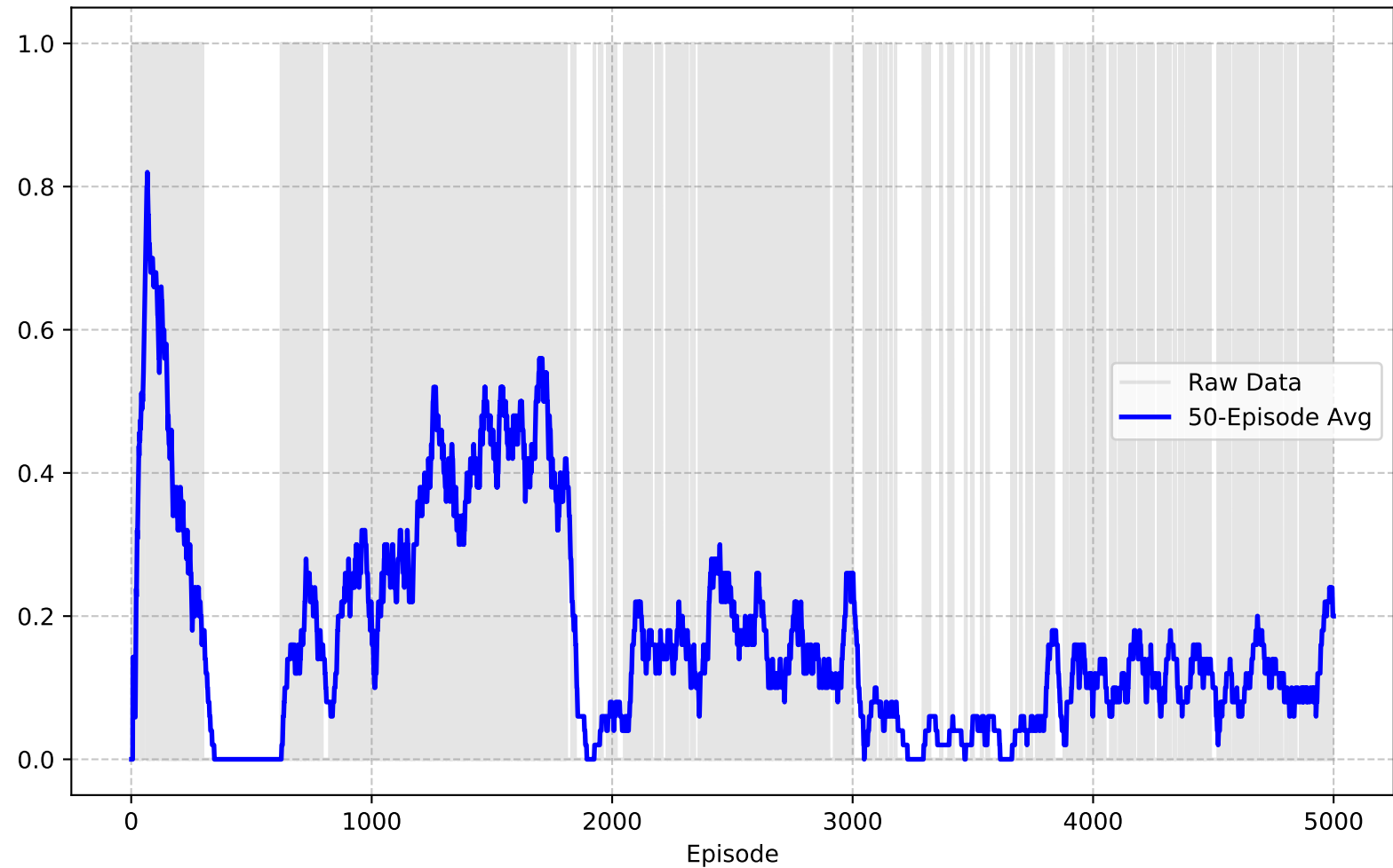
Timeout Rate (Average 50 Episodes) (Episodes 1-5000)
