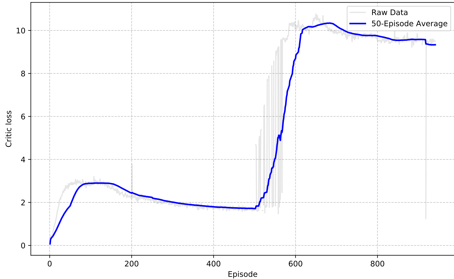
Critic loss (average 50 episodes)
