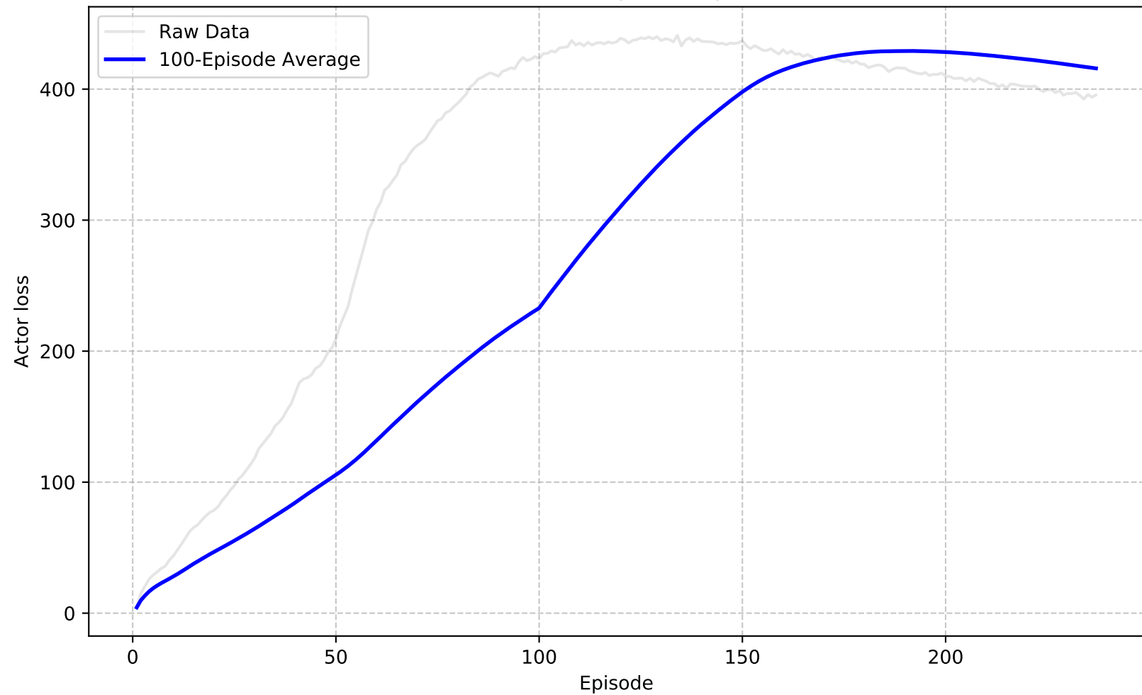
Actor loss (average 100 episodes)
