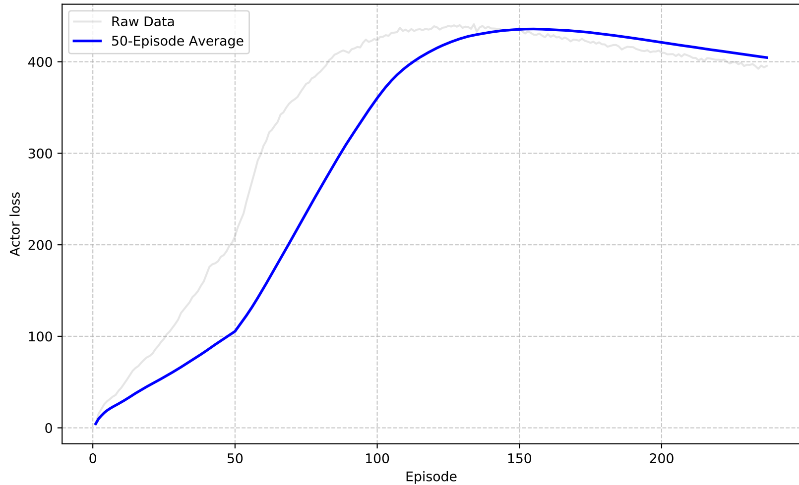
Actor loss (average 50 episodes)
