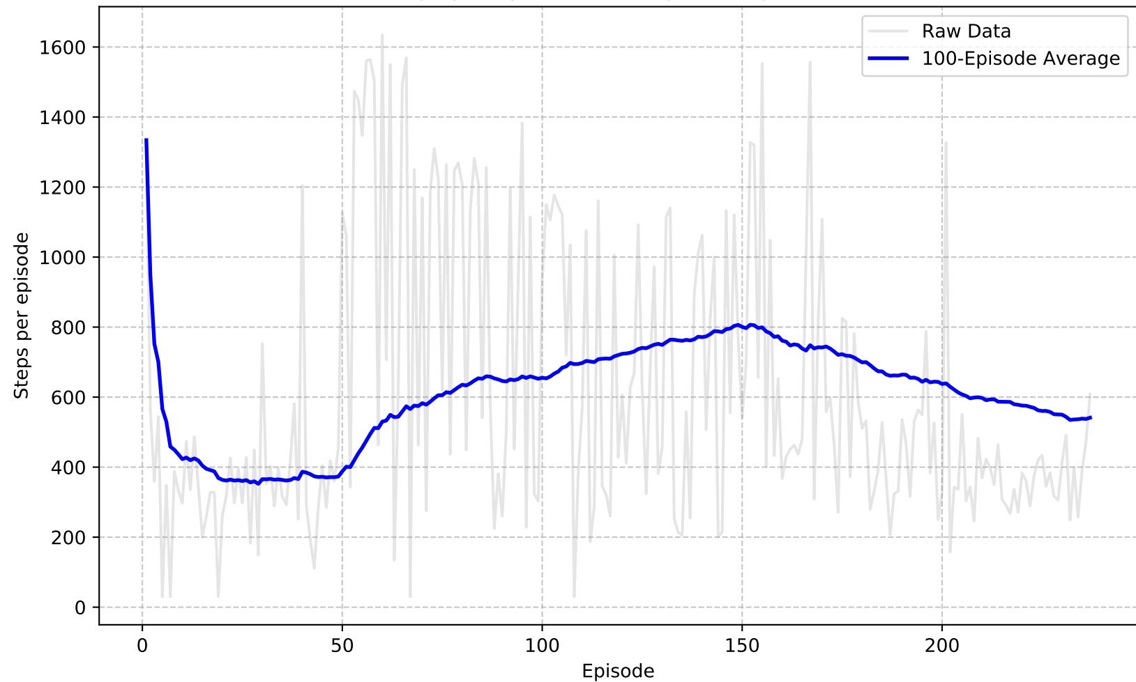
Steps per episode (average 100 episodes)
