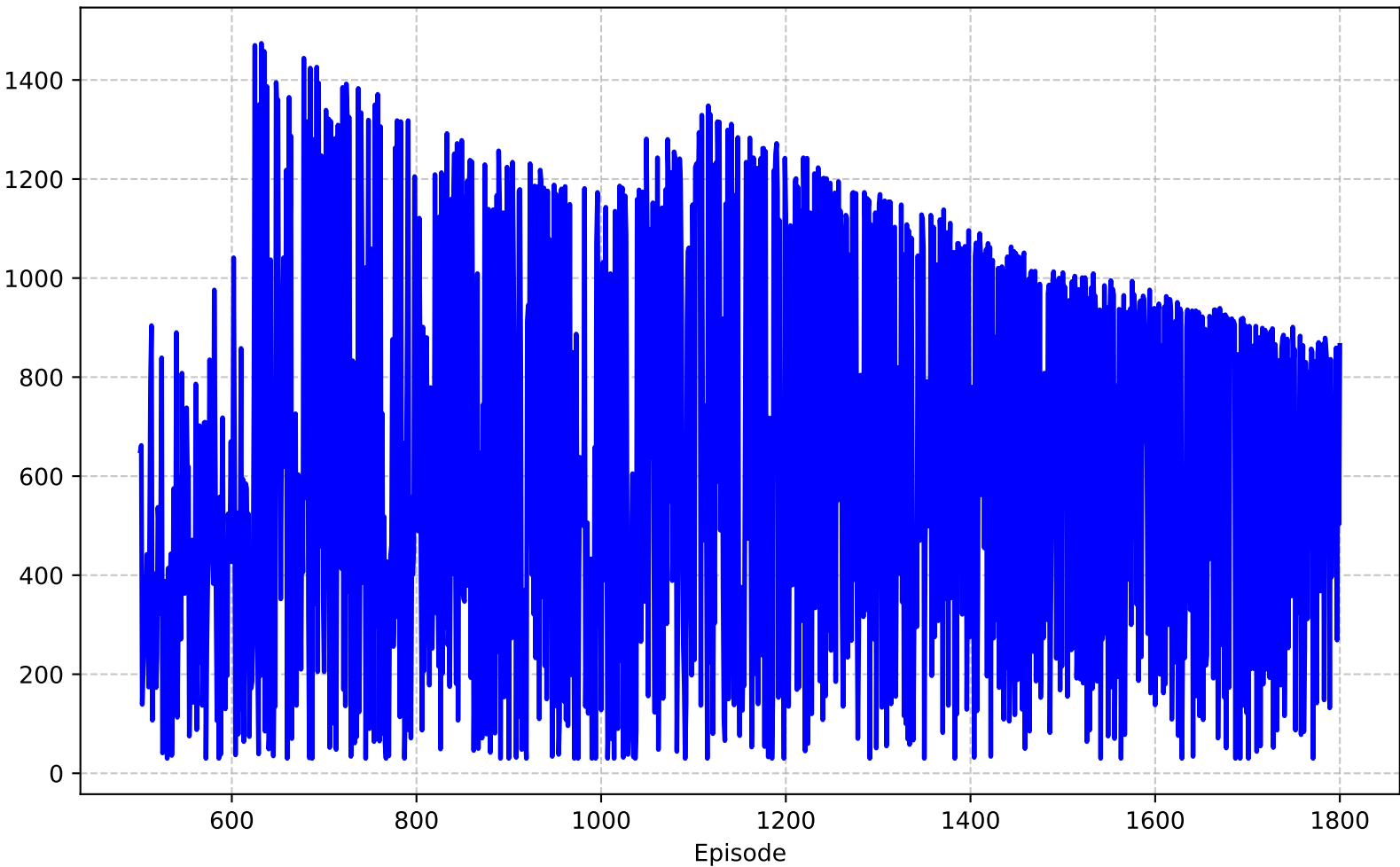
Steps Per Episode (Episodes 501-1800)
