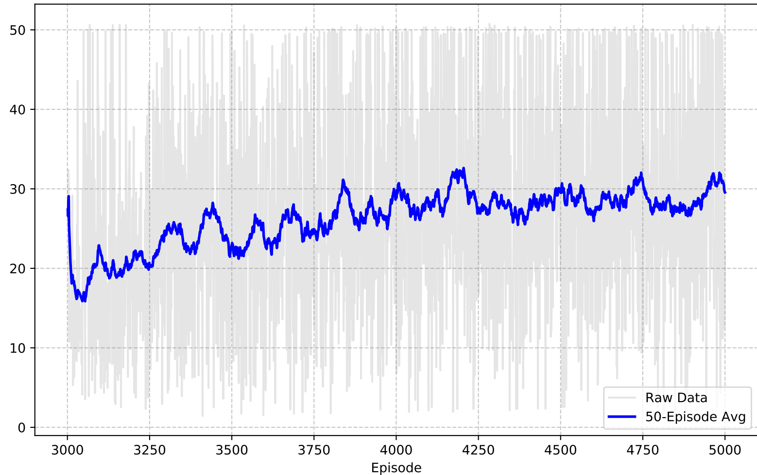
Average Duration (Average 50 Episodes) (Episodes 3001-5000)
