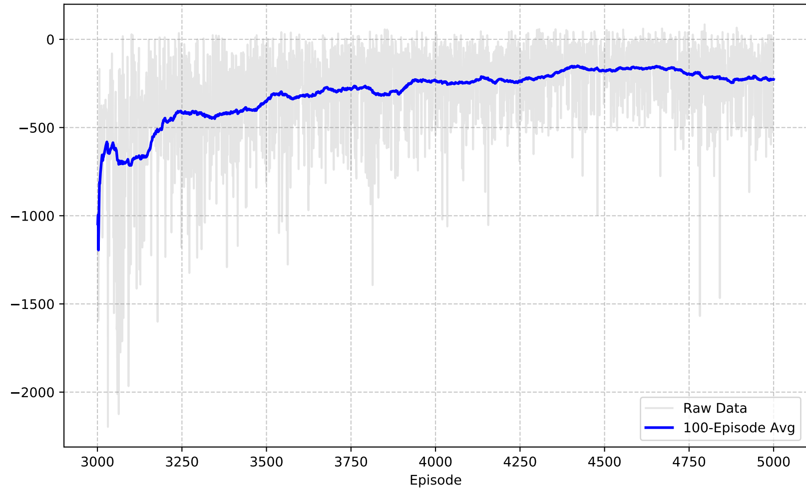
Average Reward (Average 100 Episodes) (Episodes 3001-5000)
