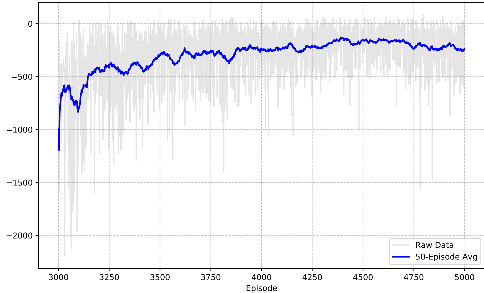
Average Reward (Average 50 Episodes) (Episodes 3001-5000)
