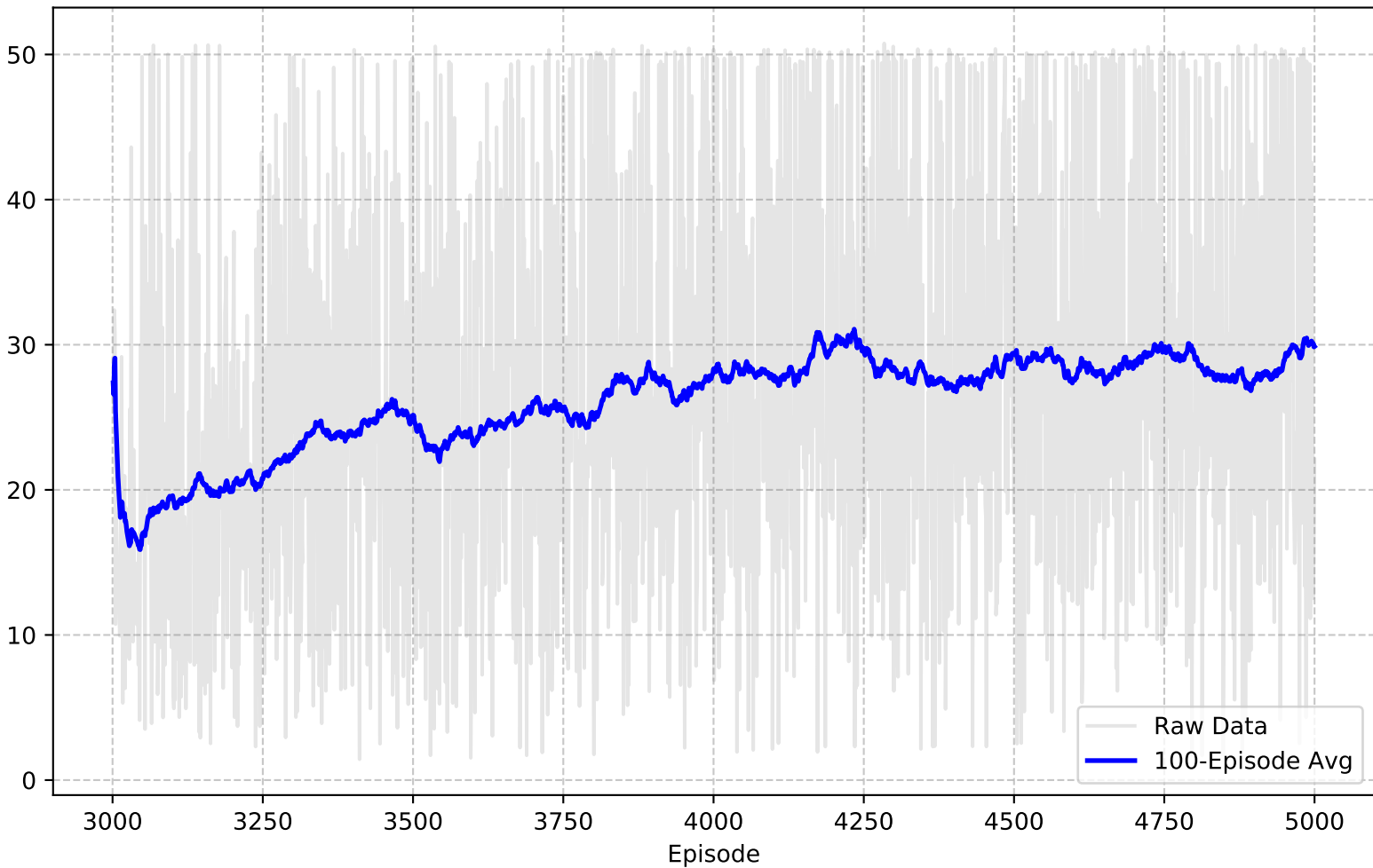
Episode Duration (Average 100 Episodes) (Episodes 3001-5000)
