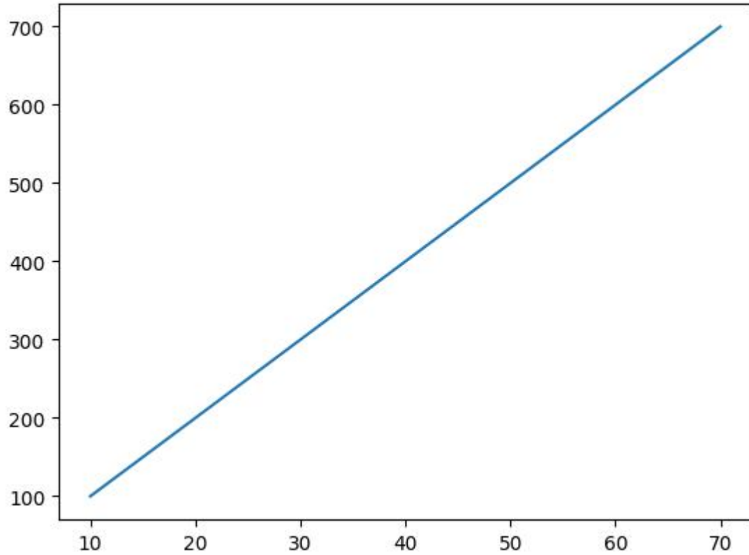
Line Plot
