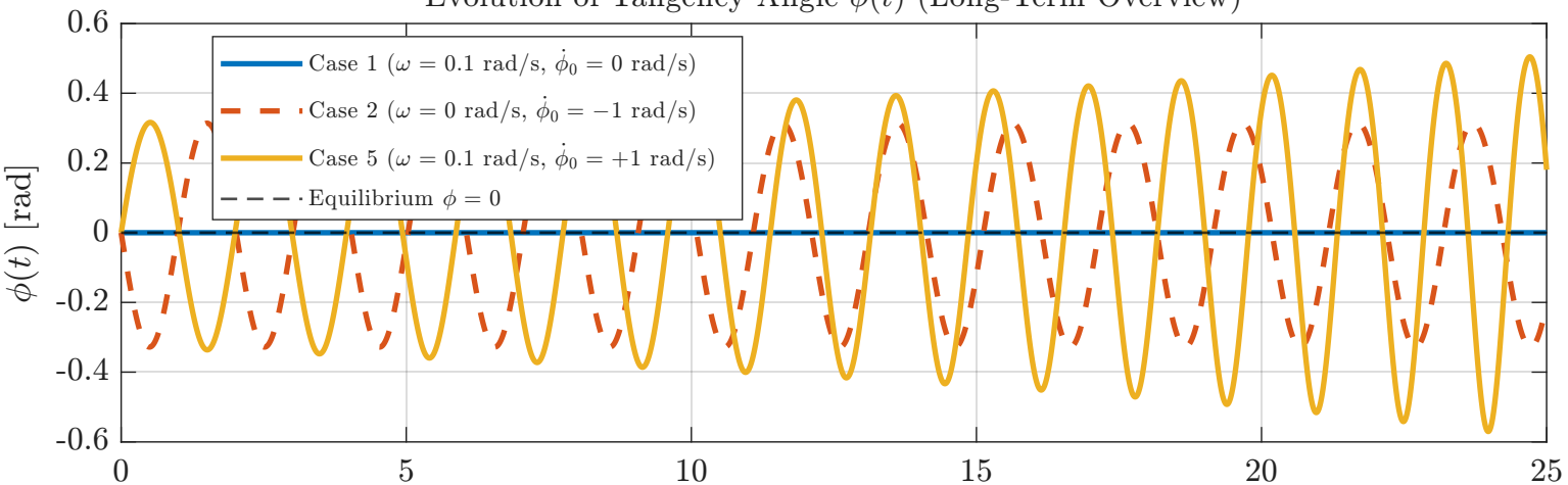
Evolution of Tangency Angle \phi(t) (Long-Term Overview)
