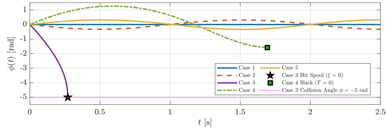
Evolution of Tangency Angle \phi(t) (Short-Term Transients, t \leq 2.5 s)
