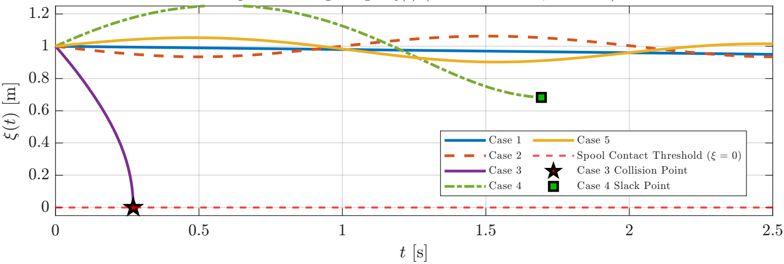
Unspooled String Length \xi(t) (Transient Phase, t \leq 2.5 s)
