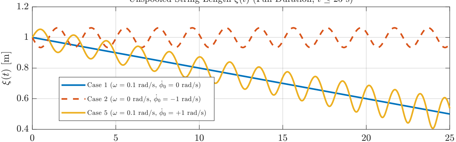
Unspooled String Length \xi(t) (Full Duration, t \leq 25 s)
