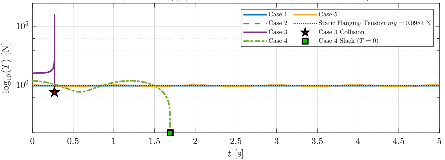
String Tension T(t) (Logarithmic Scale showing Singularity Spike)
