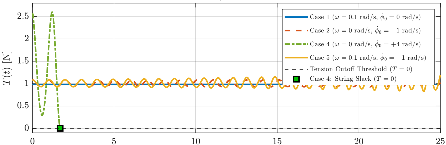
String Tension T(t) for Cases 1, 2, 4, and 5
