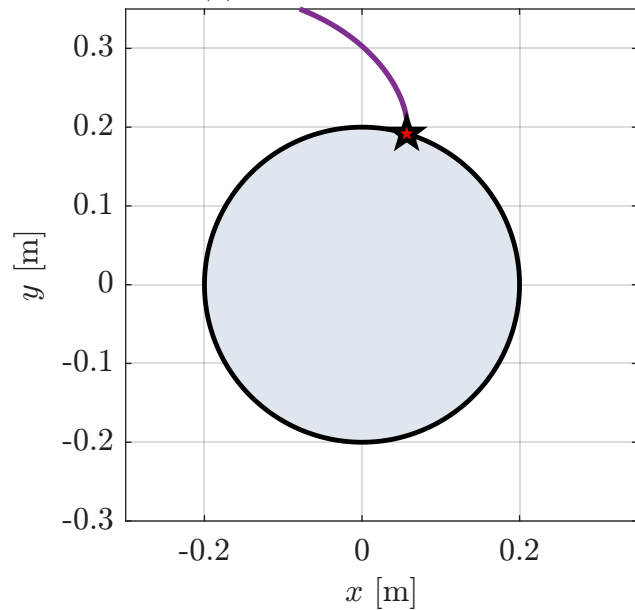
(a) Inward Spiral Trajectory
