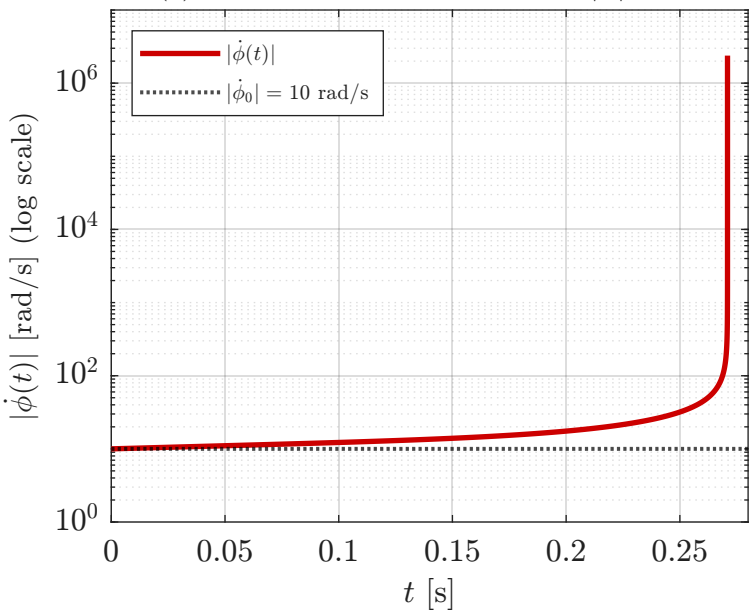
(c) Angular Velocity Singularity |\dot{\phi}| \rightarrow \infty
