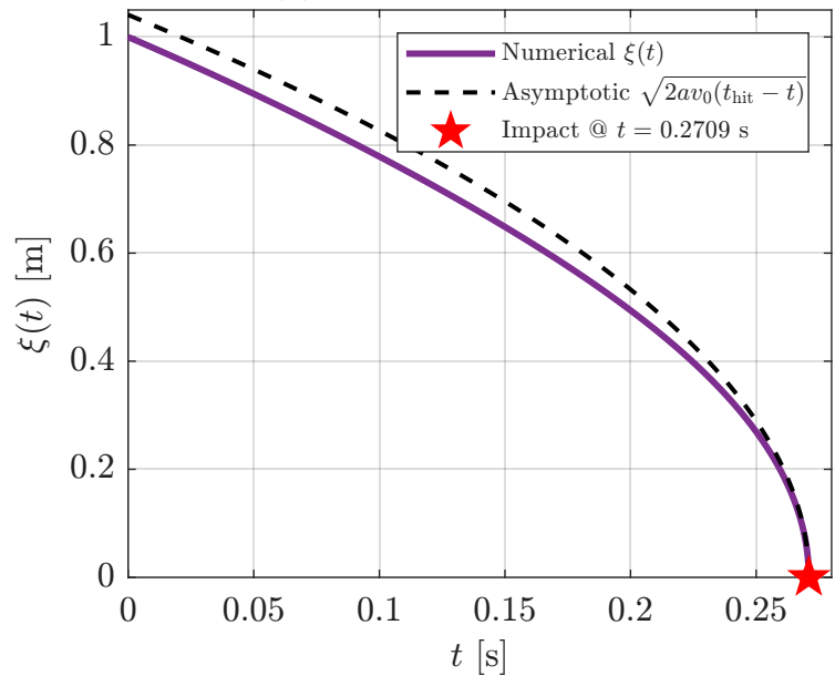
(b) Unspooled Length \xi \rightarrow 0
