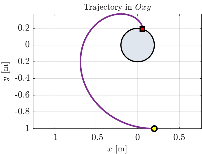
Case 3: Comprehensive Dynamics Summary ( \omega = 0 rad/s, \dot{\phi}_0 = -10 rad/s)
