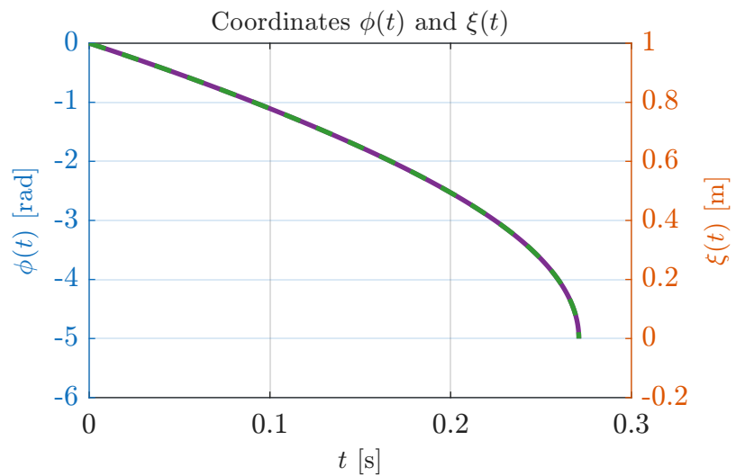
Case 3: Comprehensive Dynamics Summary ( \omega = 0 rad/s, \dot{\phi}_0 = -10 rad/s)
