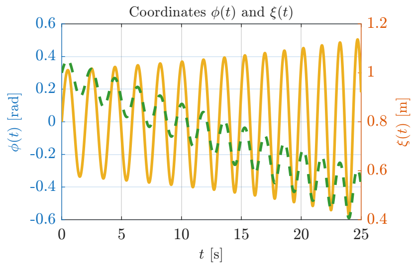
Case 5: Comprehensive Dynamics Summary ( \omega = 0.1 \text{ rad/s} , \dot{\phi}_0 = +1 \text{ rad/s} )
