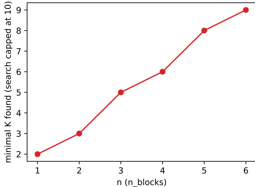
Diverging blocks: minimal K grows with n
