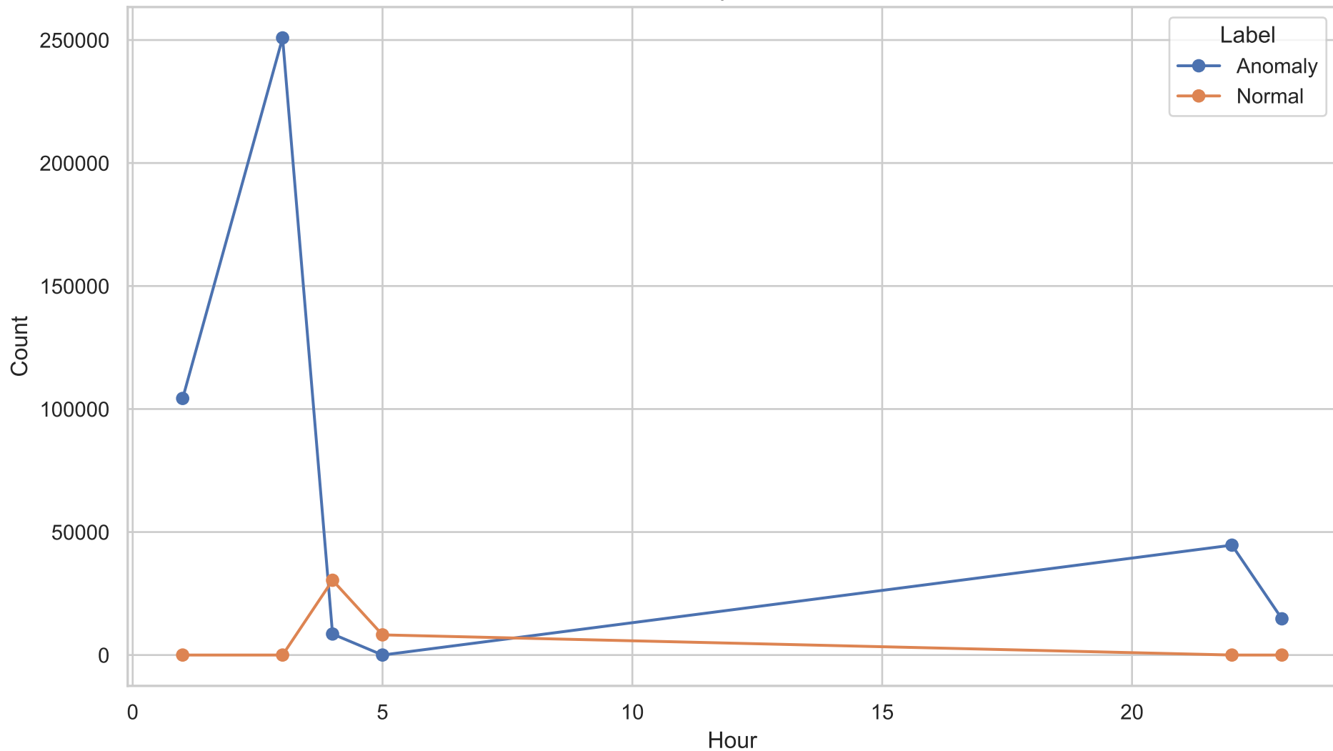
Traffic Count by Hour and Label
