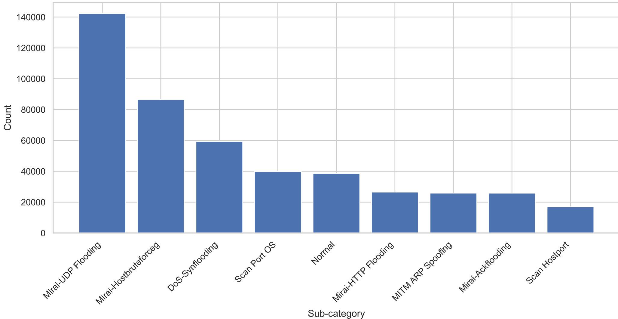
Attack Sub-Category Distribution
