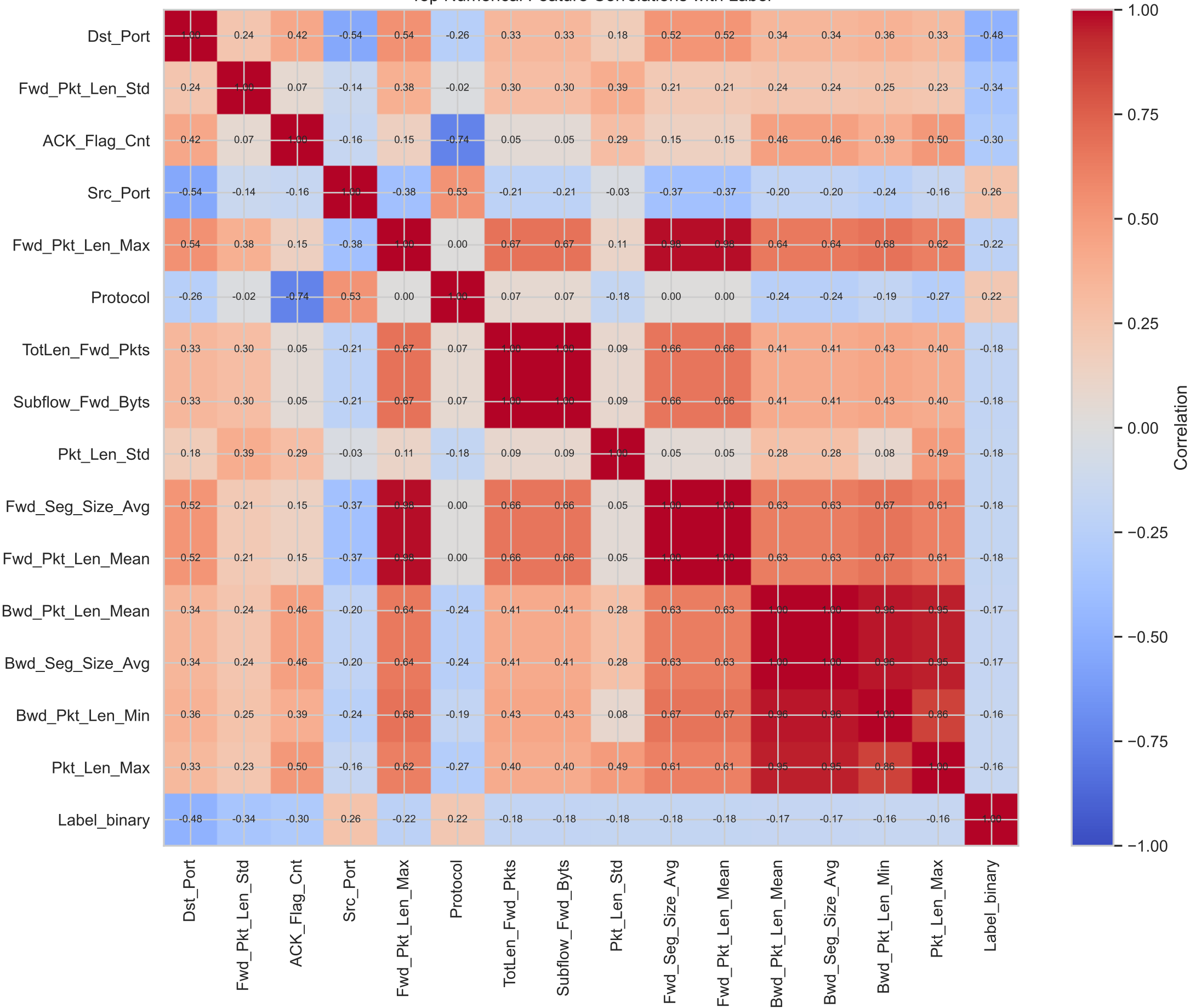
Top Numerical Feature Correlations with Label
