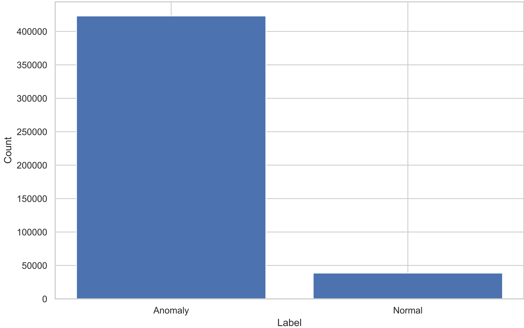
Label Distribution
