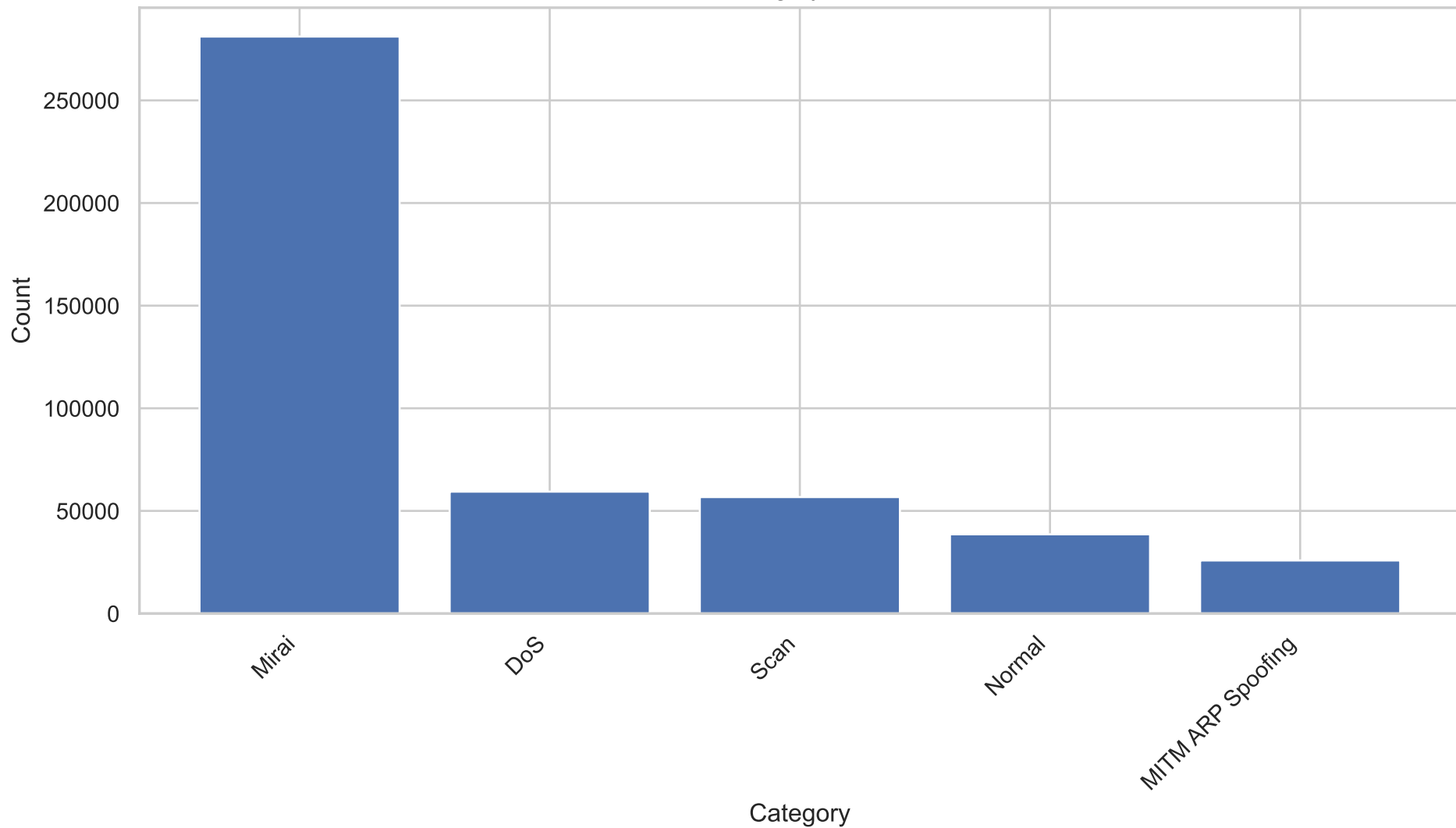
Attack Category Distribution
