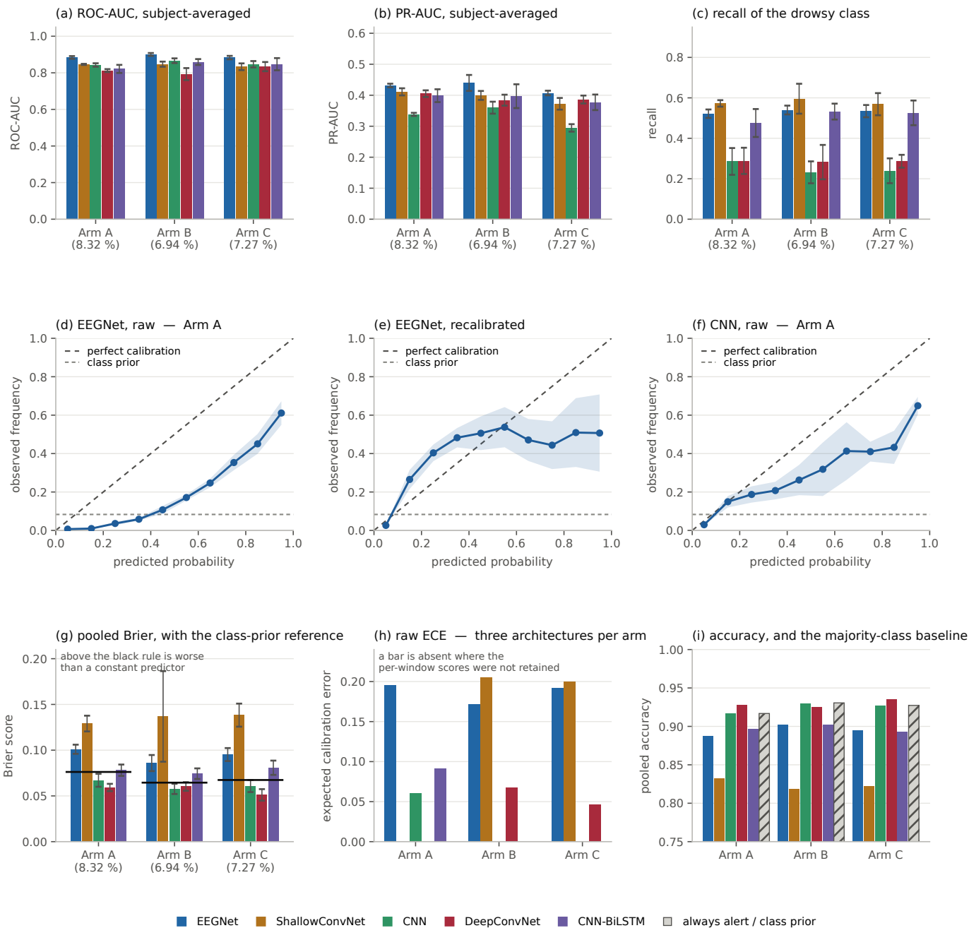
Five architectures, three window-set constructions, leave-one-subject-out bars follow the legend order left to right within every group; error bars are the standard deviation across the five seed-level means
