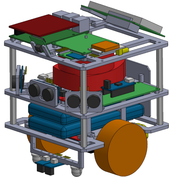
Fig. 1. Implemented autonomous robot platform [3]
